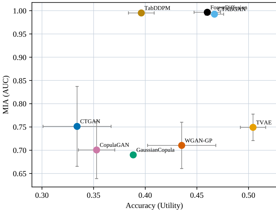
Wine Quality: Accuracy (Utility) vs MIA (AUC)
